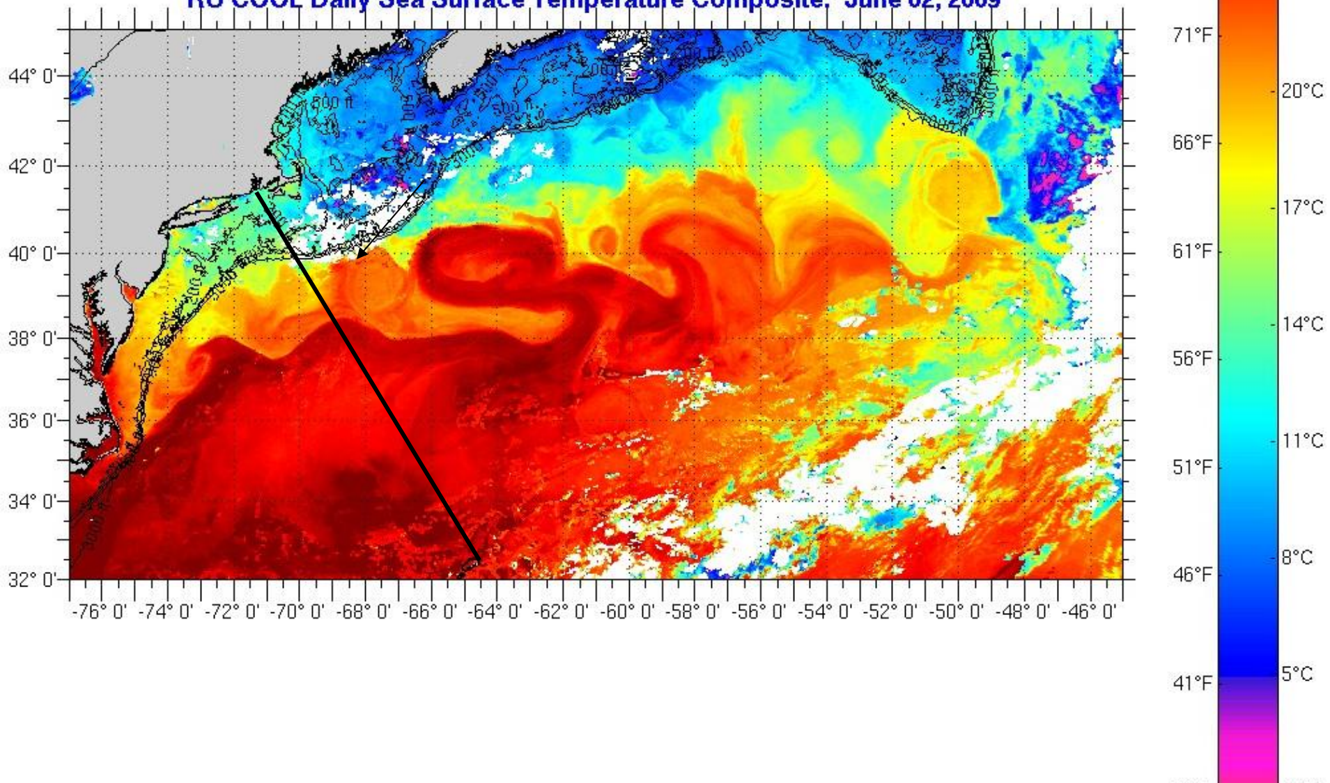
RU COOL Daily Sea Surface Temperature Composite: June 02, 2009
