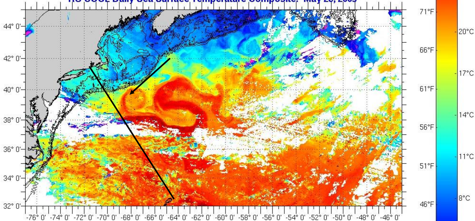
Figure 4 Satellite Sea One Day Surface Temperature Composite
